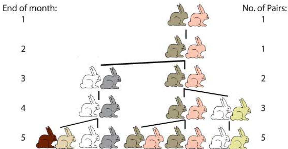
Figure 7.5: https://learnodo-newtonic.com/wp-content/uploads/2015/09/Fibonacci-Sequence-in-the-Rabbit-Problem.jpg
